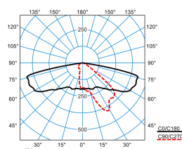
9301K AB2L-SLR2/1650-730 4G3 ET(CLO end value)
