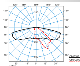
9301K AB2L-SLR2/1650-730 4G3 ET(CLO initial value)
