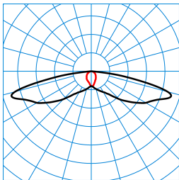
LIQ 50N-SB3L-LRA/1000-730 2G1 ETDD (CLO initial value) TX779800
