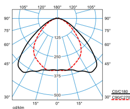
ELINE LVW55-140 ML 865 L225 4 50
