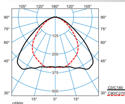
ELINE LVW55-140 ML 865 L225 0 50
