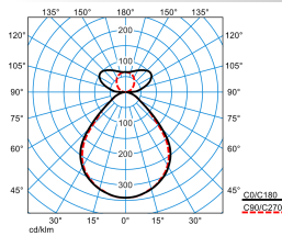
Opendo H1-L PW19 20-53/6/ML-830 ET 03 (1900lm)
