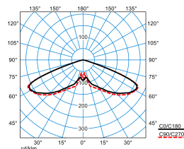
Publisca P2-RB6L/3500-740 4G1S ETDD (CLO end value)
