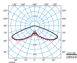
Publisca P2-RB6L/3500-740 4G1S ETDD (CLO initial value)
