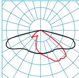
LIQ 70N-AB7L-LR/15000-740 12G1 ET(CLO end value) TX277959 ■ C0 - C180 ■ C90 - C270 DIN 5040: A30 UTE: 1,00 E DLOR: 100 % ULOR: 0 % CEN Flux Code: 39 76 98 100 100
