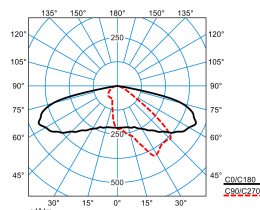
LIQ 50N-AB2L-LRA/6200-727 6G1 ETDD (CLO end value)
