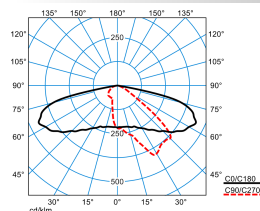
LIQ 50N-AB2L-LRA/6200-727 6G1 ETDD (CLO initial value)
