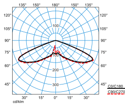
Publisca P1W-RB6L/2200-730 3G1S
