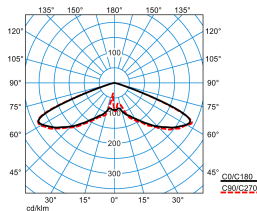
Publisca P1W-RB6L/2200-730 3G1S ETDD (CLO end value)
