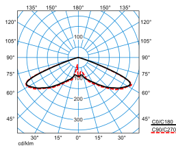
Publisca P1W-RB6L/2200-730 3G1S ETDD (CLO initial value)
