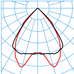
SFlow D1-L MRX LED3200-830 ETDD 03 TX769870
