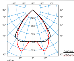
SFlow D1-L MRX LED3200-830 ETDD 03 TX769870
