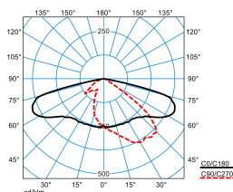
LIQ 70N-AB7L-LRA/6800-730 8G1 ETDD(CLO initial value) TX278277
