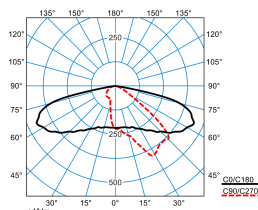
LIQ 50N-AB2L-LRA/6800-727 6G1 ETDD (CLO end value)
