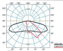
LIQ 50N-AB2L-LRA/6800-727 6G1 ETDD (CLO initial value)
