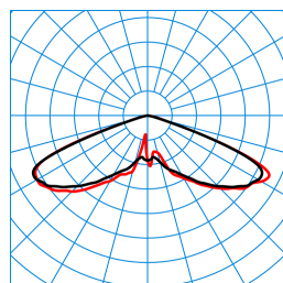
Publisca P2-RB6L/2000-740 3G1S ETDD (CLO initial value) TX300622 ■ C0 - C180 ■ C90 - C270 DIN 5040: A20 UTE: 1,00 J DLOR: 100 % ULOR: 0 % CEN Flux Code: 20 57 98 100 100
