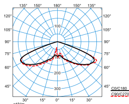
Publisca P2-RB6L/2000-740 3G1S ETDD (CLO end value) TX300731 DIN 5040: A20 UTE: 1,00 J DLOR: 100 % ULOR: 0 % CEN Flux Code: 20 57 98 100 100
