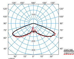
Publisca P2-RB6L/2000-740 3G1S ETDD (CLO end value)
