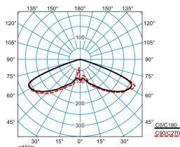
Publisca P2-RB6L/2000-740 3G1S ETDD (CLO initial value) TX300622 DIN 5040: A20 UTE: 1,00 J DLOR: 100 % ULOR: 0 % CEN Flux Code: 20 57 98 100 100
