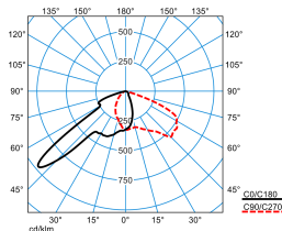
LIQ 70N-FL1L/6800-730 8G1 ET(CLO end value) TX277772
