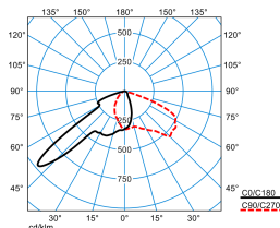
LIQ 70N-FL1L/6800-730 8G1 ET(CLO initial value) TX277714
