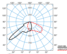
LIQ 70N-FL1L/6800-730 8G1 ET(CLO end value)
