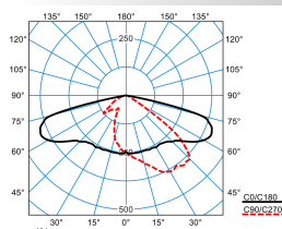
LIQ 70N-AB7L-LRA/16000-730 12G1 ETDD (CLO initial value)
