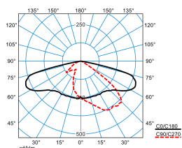
LIQ 70N-AB7L-LRA/16000-730 12G1 ETDD (CLO initial value) TX778582
