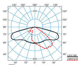
LIQ 70N-AB7L-LRA/16000-730 12G1 ETDD (CLO end value)
