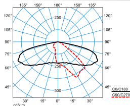
LIQ 50N-AB2L-SLR2/6800-722 6G1 ET (CLO initial value)
