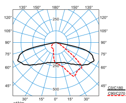
LIQ 50N-AB2L-SLR2/6800-722 6G1 ET (CLO initial value) TX777280
