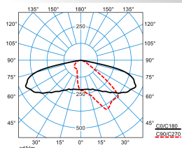
LIQ 50N-AB2L-SLR2/6800-722 6G1 ET (CLO end value) TX777275
