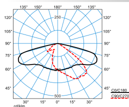
LIQ 70N-AB7L-LR/8200-740 10G1 ET(CLO initial value)
