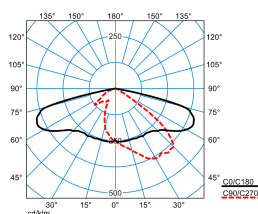
LIQ 70N-AB7L-LR/8200-740 10G1 ET(CLO end value)
