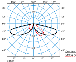
CS 19 100-AB2L/1650-730 2G1S ETDD (CLO initial value)
