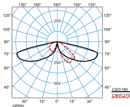
CS 19 100-AB2L/1650-730 2G1S ETDD (CLO end value)
