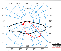
LIQ 70N-AB7L-SLR2/13000-722 12G1 ET (CLO initial value)
