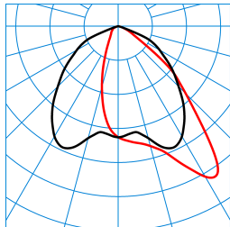
Jovie 70I-AM3L-MLLR/75-150-730 12G1 ETDD (CLO initial value) TX780167
