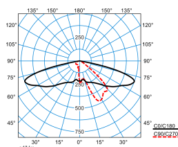
Publisca P1W-AB2L/2600-730 3G1S ETDD (CLO end value)
