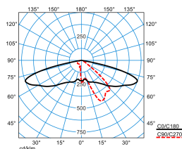
Publisca P1W-AB2L/2600-730 3G1S ETDD (CLO initial value)
