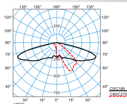
Publisca P1W-AB2L/2600-730 3G1S
