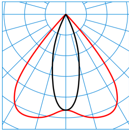
GradoTW 3P WRS-GZ 2x50-EW M50 ETBLE 01 TX870463
