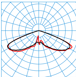
Publisca P2-RB6L/2000-730 3G1S ETDD (CLO end value) TX301916 ■ C0 - C180 ■ C90 - C270 DIN 5040: A20 UTE: 1,00 J DLOR: 100 % ULOR: 0 % CEN Flux Code: 20 57 98 100 100
