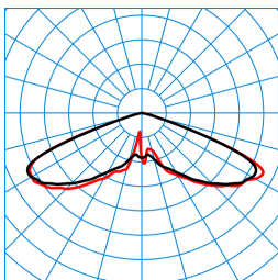
Publisca P2-RB6L/2000-730 3G1S ETDD (CLO initial value) TX301295 ■ C0 - C180 ■ C90 - C270 DIN 5040: A20 UTE: 1,00 J DLOR: 100 % ULOR: 0 % CEN Flux Code: 20 57 98 100 100
