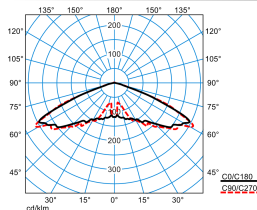
Publisca P1W-RB6L-LRA/1200-730 2G1S
