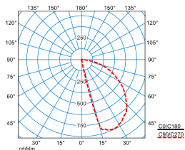
Invego Square W1 AM16L/190-940 1G1 + IP65 24V DC 10W TX120561
