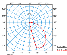
Invego Square W1 AM16L/190-940 1G1 + IP66 24V DC 20W TX120572
