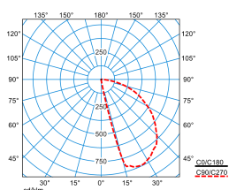
Invego Square W1 AM16L/190-940 1G1 + IP66 24V DC 40W TX120562
