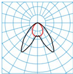
ELINE FL HE+ LDAW140 840 L225 1 20 ■ C0 - C180
