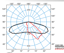
LIQ 50N-AB2L-LR-SLR2/6800-730 6G1 ET (CLO initial value)
