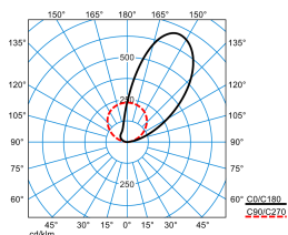
Altigo G2 60 WO GS AM15L/350-830 + VE IP66 24V DC 60W
