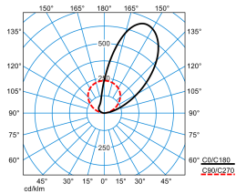
Altigo G2 60 WO GS AM15L/350-830 + VE IP66 24V DC 250W
