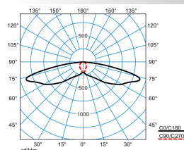
LIQ 50N-SB3L-LR/1350-727 2G1 ET (CLO initial value)
