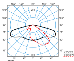
LIQ 70N-AB7L-SLR1/7500-727 8G1 ET(CLO initial value) TX278269 DIN 5040: A30 UTE: 1,00 E DLOR: 100 % ULOR: 0 % CEN Flux Code: 39 76 98 100 100
