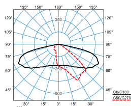
LIQ 50N-AB2L-LRA/35/42/46-740 6G1 ETDD (CLO end value)
