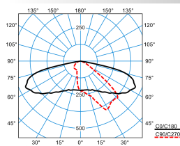
LIQ 50N-AB2L-LRA/35/42/46-740 6G1 ETDD (CLO initial value)
