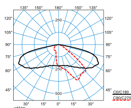
LIQ 50N-AB2L-LR-SLR2/2200-740 2G1 ET (CLO end value)
