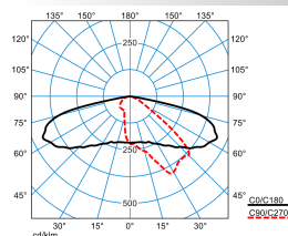
LIQ 50N-AB2L-LR-SLR2/2200-740 2G1 ET (CLO initial value)
