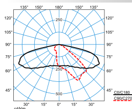
LIQ 50N-AB2L-LR-SLR2/2200-740 2G1 ET (CLO initial value)
