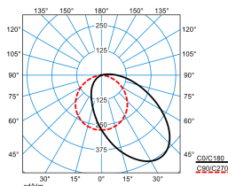
Sanesca W3-S2/R LED5000-840 01 (reading_light)
