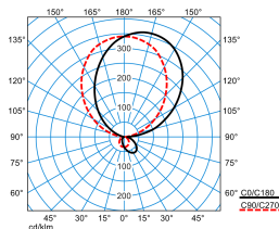
Sanesca W3-S2/R LED5000-840 01
