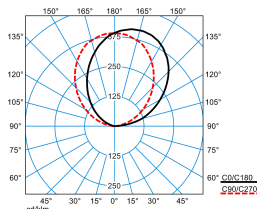
Sanesca W3-S2/R LED5000-840 01 (room_light)
