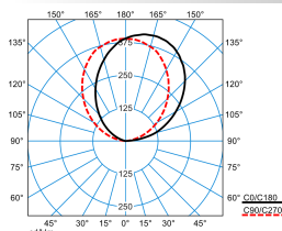
Sanesca W3-S2/R LED5000-840 01 (night_light)
