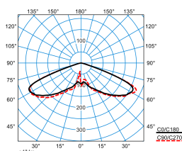
Publisca P2-RB6L-LR/2000-730 3G1S ET (CLO initial value) TX300498 DIN 5040: A20 UTE: 1,00 J DLOR: 100 % ULOR: 0 % CEN Flux Code: 20 57 98 100 100
