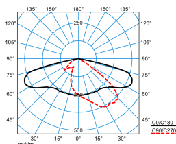
LIQ 70N-AB7L-LR/75/82/91-730 10G1 ET(CLO initial value) TX277798
