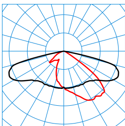
LIQ 70N-AB7L-LR/75/82/91-730 10G1 ET (CLO initial value) TX277798 DIN 5040: A30 UTE: 1.00 E DLOR: 100 % ULOR: 0 % CEN Flux Code: 39 76 98 100 100
