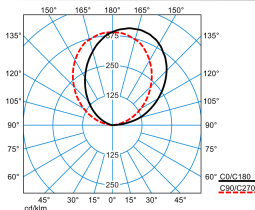
Sanesca W3-S2/R LED5000-830 01 (night light)
