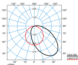
Sanesca W3-S2/R LED5000-830 01 (reading light)
