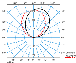
Sanesca W3-S2/R LED5000-830 01 (room light)
