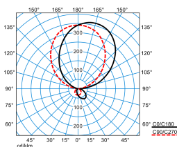
Sanesca W3-S2/R LED5000-830 01
