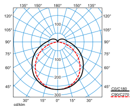
Deveo G3 15 DL 41-80/3ML-8MC ET PC +LV (stage 4)
