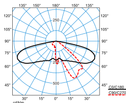
Publisca P2-AB2L-LRA/2600-730 3G1S ET (CLO initial value) TX301310 DIN 5040: A30 UTE: 1,00 l DLOR: 100 % ULOR: 0 % CEN Flux Code: 34 71 96 100 100
