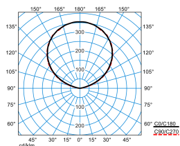
Parella H-L 13000-840 +LM1 +LLWS 01 (indirect) TX059612
