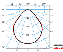
Parella H-L 13000-840 +LM1 +LLWS 01 (direct c270geo) TX059618
