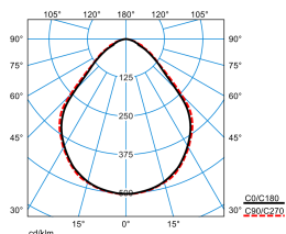
Parella H-L 13000-840 +LLWS 01 (direct c90geo) TX057112
