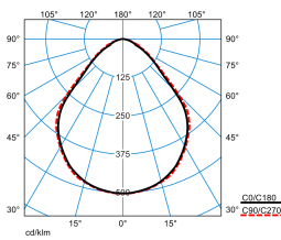
Parella H-L 13000-840 +LM1 +LLWS 01 (direct c90geo) TX059619
