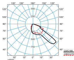
LIQ 50N-FR1L/5600-727 6G1 ET (CLO initial value) TX780644
