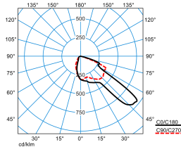
LIQ 50N-FR1L/5600-727 6G1 ET (CLO end value) TX780638
