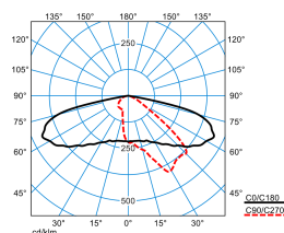
LIQ70N-AB2L12S2-76-7TW-ET-CAB-26 (DCW-CLO initial value)
