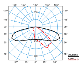
LIQ70N-AB2L12S2-76-7TW-ET-CAB-26 (DCW-CLO end value)
