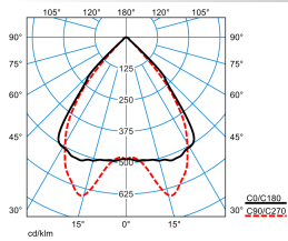
SFlow D1-L MRX LED3200-830 ET 03 TX769857
