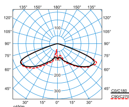
Publisca P2-RB6L-LR/2000-740 3G1S ET (CLO end value) TX301894 DIN 5040: A20 UTE: 1,00 J DLOR: 100 % ULOR: 0 % CEN Flux Code: 20 57 98 100 100
