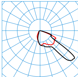
LIQ 50N-FR1L/4200-740 4G1 ET (CLO end value) TX780607 ■ C0 - C180 ■ C90 - C270 DIN 5040: A40 UTE: 1,00 F DLOR: 100 % ULOR: 0 % CEN Flux Code: 41 83 99 100 100
