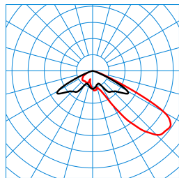
LnPlus 40-AM19L/3200-740 4G1 ETDD (CLO initial value) TX376945 ■ C0 - C180 ■ C90 - C270 DIN 5040: A30 UTE: 1,00 J DLOR: 100 % ULOR: 0 % CEN Flux Code: 26 78 99 100 100
