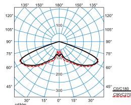
Publisca P2-RB6L/2900-730 4G1S ETDD (CLO end value)
