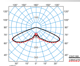
Publisca P2-RB6L/2900-730 4G1S
