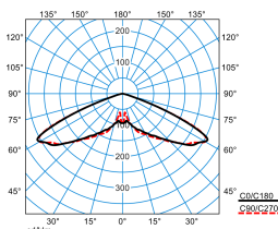
Publisca P1W-RB6L-LR/4600-730 6G1S ET (CLO initial value) TX300790
