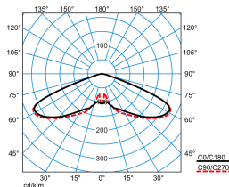
Publisca P2-RB6L-LRA/4200-740 6G1S TX047910
