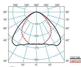
ELINE LVW40-110 ML 840 L150 4 20
