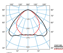
ELINE LVW40-110 ML 840 L150 2 20
