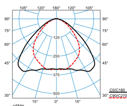
ELINE LVW40-110 ML 840 L150 4 20
