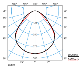
ValineoG4 M73 PW19 38-50/4ML-840 ETDD (stage 4)
