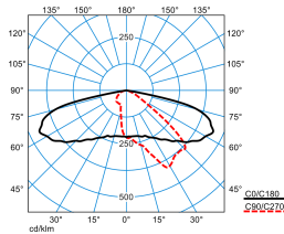
LIQ 50N-AB2L-SLR1/2200-727 2G1 ET (CLO initial value)
